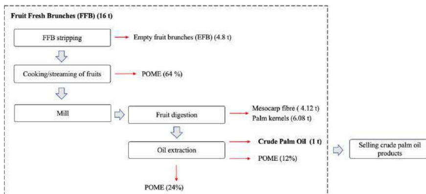
Figure 1 Crude Palm Oil processing processes.
