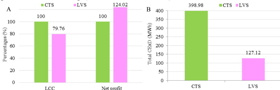
Figure 2. Comparison analysis between conventional tunnel systems (CTS) and LED-equipped vertical systems (LVS) scenarios from economical (A) and cumulative exergy demands (CExD; B) perspective.
