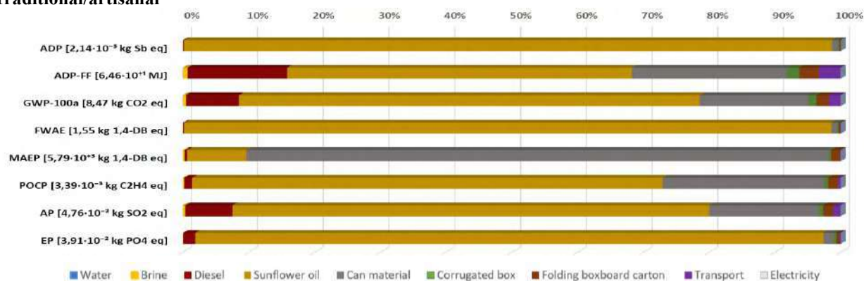
Figure 2. Comparison of the relative contributions for the canned tuna by industrial and traditional processing for 1kg of end-product.
